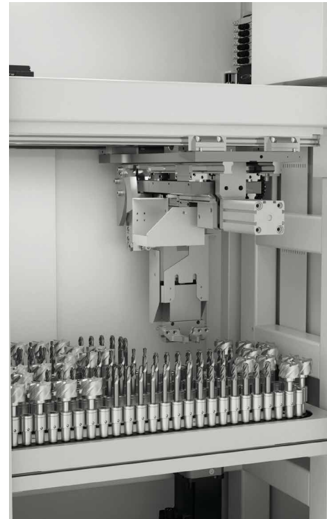
///// HC 4 AND HC 4 PLUS CHAIN MAGAZINE in compact design
