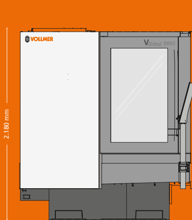
/////// MACHINE DIMENSIONS VGrind 360S without automation
