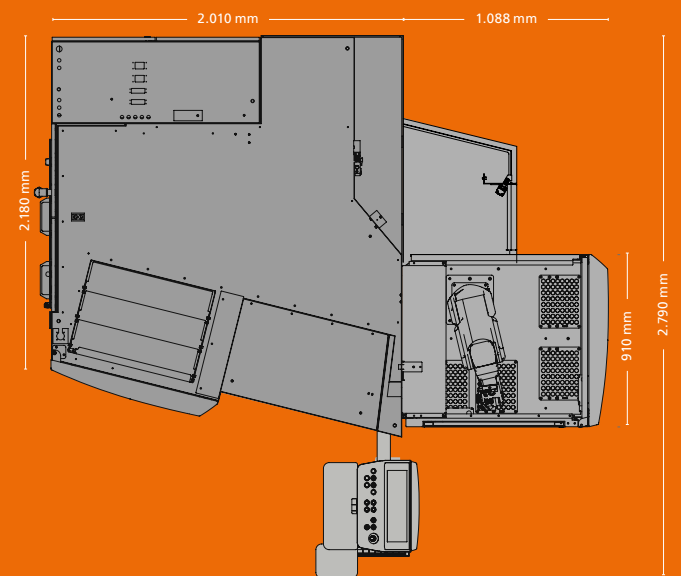
/////// MACHINE DIMENSIONS VGrind 360S with HPR 250
