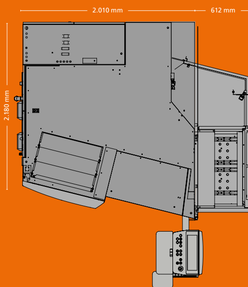
/////// MACHINE DIMENSIONS VGrind 360S with HP 170 or HC 4
